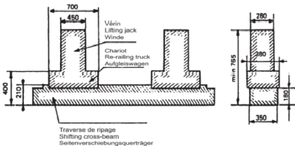
Free spaces under rerailing places
