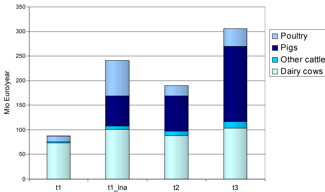
Figure 8: Additional costs (compared to the NEC-baseline case) for the IPPC extension scenarios.
